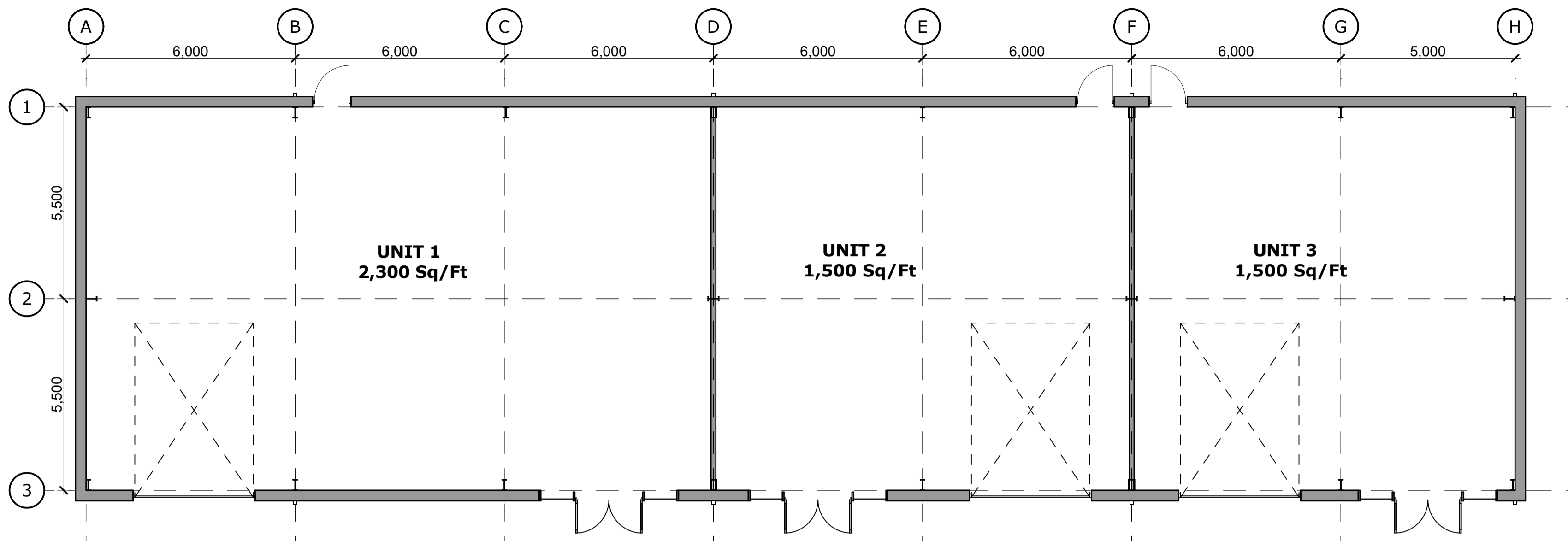
ground floor plan 1:100
