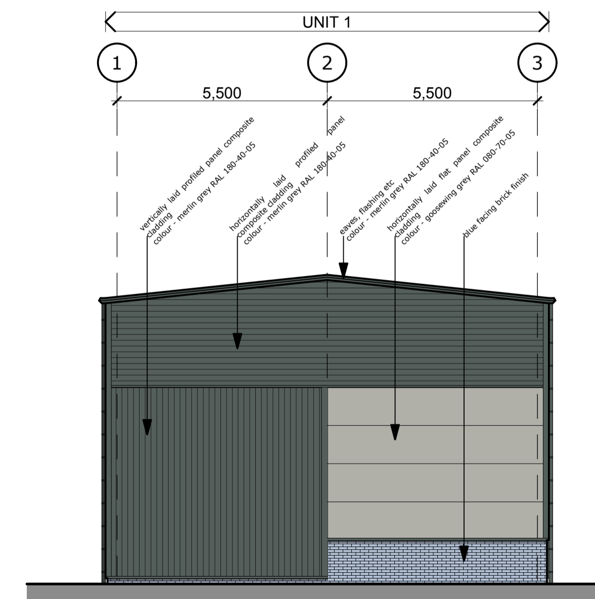
side (west) elevation 1:100
