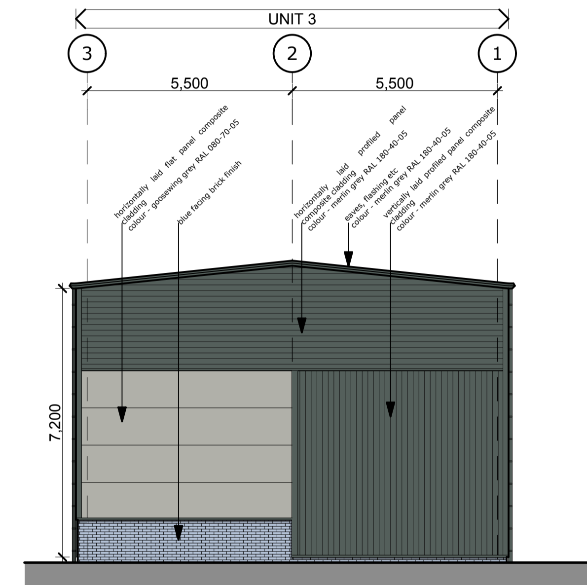
side (east) elevation 1:100
