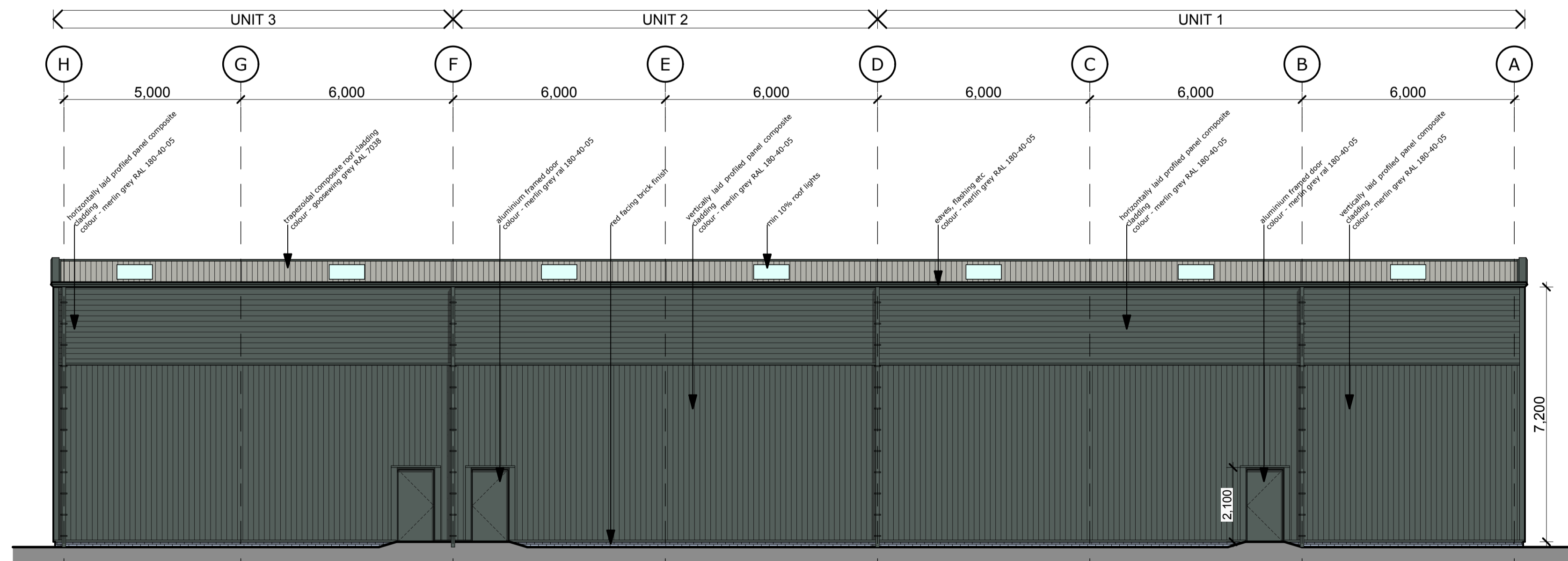
rear (north) elevation 1:100
